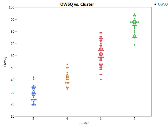
Figure 8 - Comparison of multivariate versus univariate clustering.
