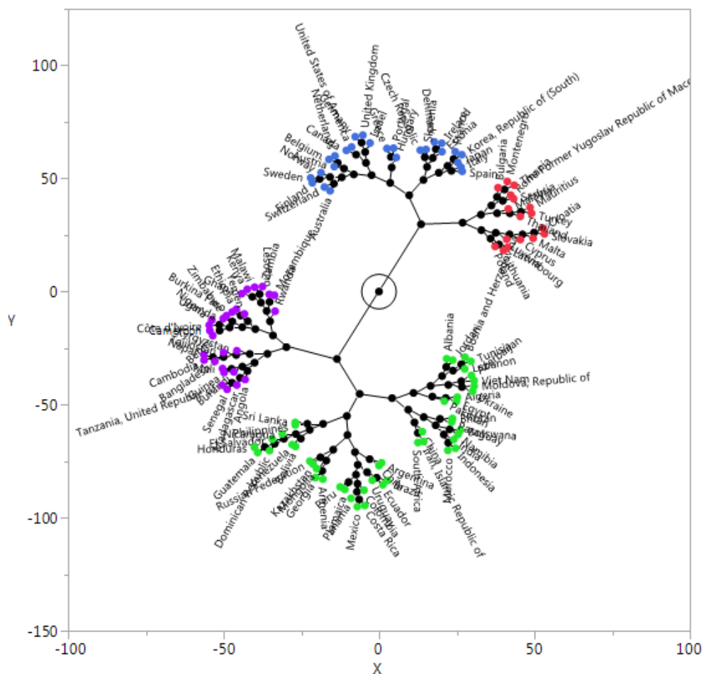
Figure 6 - Cluster constellation plot position for the 118 countries.
