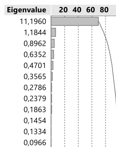
Figure 4 - PCA analysis: the successive principal components.
