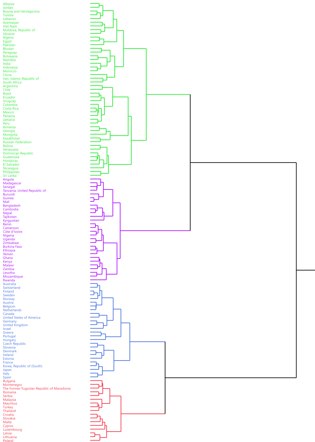
Figure 7 - Dendrogram obtained for the 118 countries using ranking values for the indicators.
